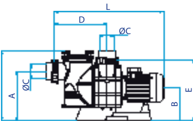
COLORADO pump with strainer Bomba COLORADO con pre-filtro
