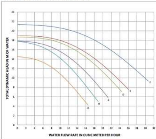
50Hz Performance Curve
